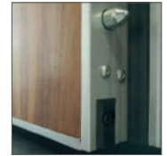
Detalle carenado inferior y 4 bulones antipalanca Detail lower fairing and 4 anti-lever bolts
